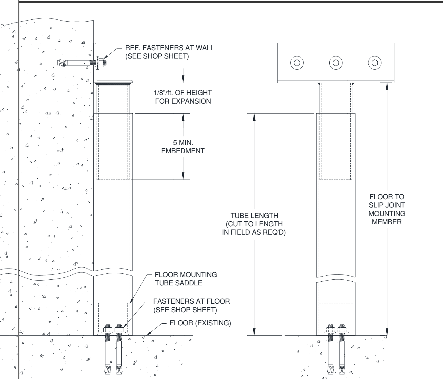
Figure 5.16 – Slip Joint - Floor to Wall with Angle Mounting Assembly
